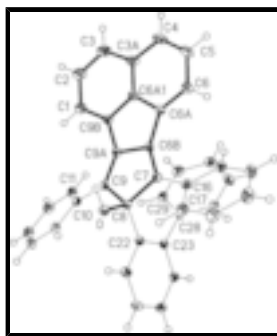
Fig. 1. The formula unit of the title compound in the crystal. Ellipsoids represent 50% probability levels. Only the first two atoms of phenyl rings are numbered; other atoms follow in sequence.
